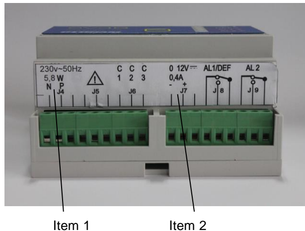
Figure 2 : power supply connections
