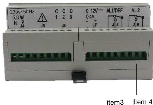
Figure 5 : relays terminals
